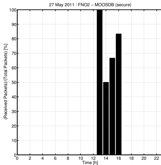
Figure 14: Packet reception ratio recorded on May 27, 2011 along the link FNO2 - MOOSDB. Network security services were activated. Variations in communication performance are clearly visible.
