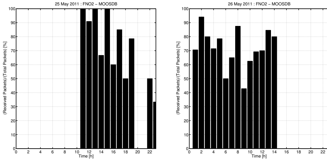
Figure 13: Packet reception ratio recorded on May 25-26, 2011 along the link FNO2 - MOOSDB. It is clearly visible the variation in the communication performance during the operation days. Network security was kept off for most of the period and activated on May 26, 2011 at 15.14pm. From this moment on FNO2 was maintained out of the network by the DB as the node was not switched to the secure communication mode, and hence considered as an intruder. It re-entered into the UAN on May 27, 2011 when it was switched to the secure IS-MOOS (see Figure 14).
