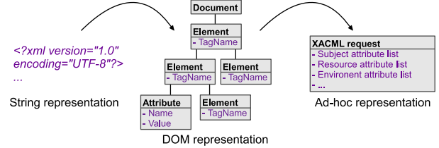
Figure 9. XML conversion
